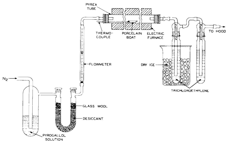
FIG. 1 Assembly of Apparatus
